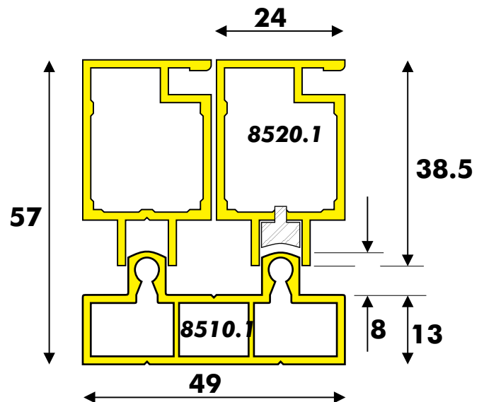
Above: Slider Inner and Outer Profile shown to scale
