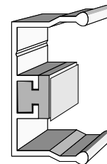
Side Guide - including magnetic strip
